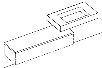
Wall-Mounted Vanity Top with faucet hole IoK URBAN Ecru 1200 × 500 × 125 mm
