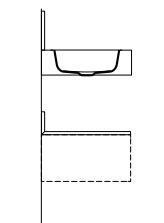
Top and Sipario backsplash IoK MOON Basalto 1800 × 450 × 12 mm 1800 × 12 × 100 mm
