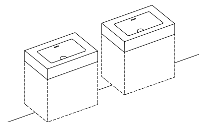
Vanity Countertop IoK SHINE Crystal White 660 × 450 × 150 mm
