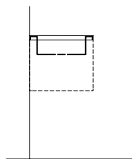
Vanity Countertop IoK IMPERIALE Calacatta Bernini 2400 × 450 × 30 mm
