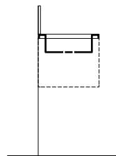
Vanity Countertop IoK IMPERIALE Port Laurent 2400 × 450 × 12 mm
