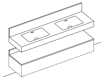
Wall-Mounted Vanity Top and Sipario backsplash with faucet holes IoK MOON Basalto 1800 × 450 × 125 mm 1800 × 12 × 200 mm
